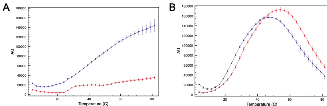
Figure 3. SLS analysis of the disulfide bound ATF5 dimer (red upright triangles) and C240A monomer (blue downturned triangles) in the absence (A) or presence (B) of 10 mM DTT as a function of temperature.
